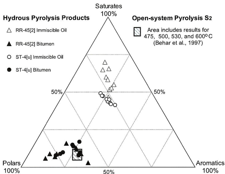
Fig. 4. Ternary diagram of C 15+ saturate, aromatic, and polar (i.e., resins + asphaltenes) fractions of immiscible oils and bitumen generated by hydrous pyrolysis for 72-h durations at 300–365 °C for samples ST-4[u] and RR-45[2]. Saturate, aromatic, and resin fractions were determined by column chromatography using alumina/silica gel (2:1 v/v) columns (0.8 × 25 cm) and eluting solvents of hexane, benzene, and benzene: methanol (1:1 v/v), respectively. Asphaltenes were precipitated with n -hexane. The boxed field denotes compositions for S 2 products generated by open-system pyrolysis at 475, 500, 530, and 600 °C as reported by Behar et al. (1997).
