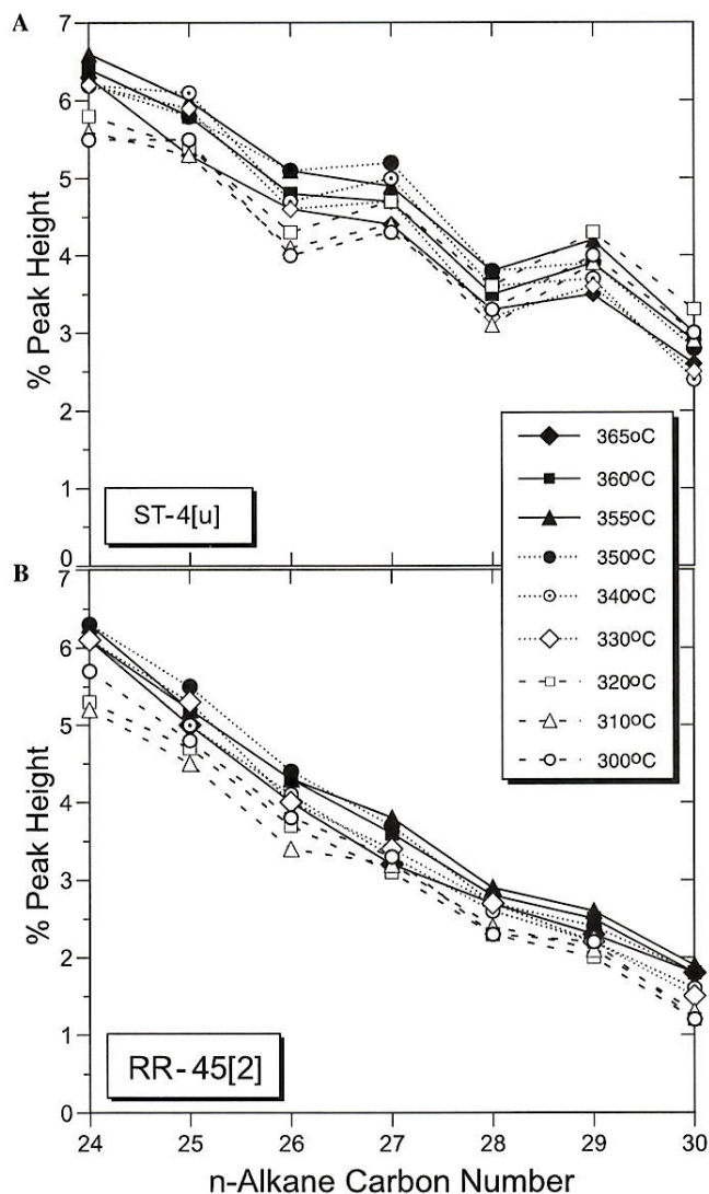
Fig. 5. Distribution of n -C 24 to n -C 30 alkanes based on normalized gas-chromatogram peak heights from n -C 17 to n -C 30 n -alkanes in immiscible oils generated by hydrous pyrolysis at 300–365 °C for 72-h durations from samples (A) ST-4[u] and (B) RR-45[2]. Immiscible oils were analyzed as whole oils in a split mode on a DB1 column of a Hewlett-Packard 6890 gas chromatograph.
