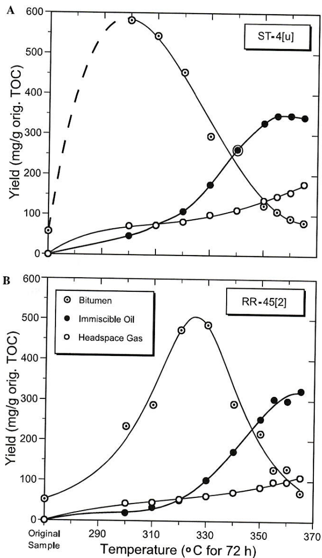
Fig. 3. Changes in hydrous-pyrolysis products generated at different temperatures (300–365 °C) for 72-h durations from samples (A) ST-4[u] and (B) RR-45[2]. Yields are calculated in milligrams of product per gram of original total organic carbon (TOC). General trend curves are best-fit polynomials with no theoretical basis. Bitumen yields were determined on pulverized (<0.2 mm) recovered rock (~10 g) that was extracted with a dichloromethane/methanol mixture (93:7 v/v) using a Soxhlet apparatus. The extraction procedure consisted of a 2-h boiling followed by a 3-h rinse. Bitumens were concentrated by evaporation of the extracting solvent at ambient temperatures under a fume-hood until a constant weight was obtained. Generated gas yields are based on gas collected from reactor headspace and analyzed on a Wasson-Ece/Hewlett-Packard 6890 gas chromatograph using two thermal conductivity detectors and one flame ionization detector.
