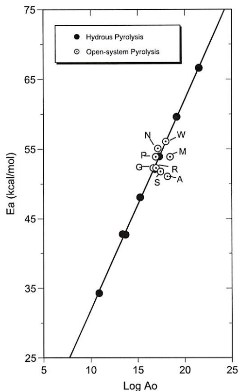
Fig. 14. Plot of mean-weighted activation energies ( E_a in kcal/mol) and log of single frequency factors ( A_o in 1/h) derived from open-system pyrolysis (open centered points) of samples ST-4[u] (S) and RR-45[2] (R) from this study, and samples of Green River Fm. (G), Woodford Shale (W), New Albany Shale (N), Phosphoria Fm. (P), Monterey Fm. (M), and Alum Shale (A) from Lewan and Ruble (2002). Solid points and line are compensation relation for kinetic parameters derived from hydrous pyrolysis as shown in Fig. 11.
