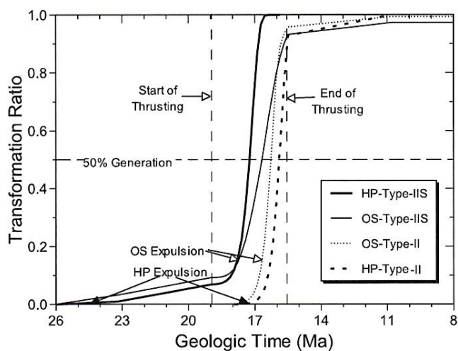
Fig. 16. Generation curves for immiscible oil generation from hydrous-pyrolysis (HP) kinetic parameters and S_2 generation from open-system pyrolysis (OS) kinetic parameters for samples ST-4[u] (Type-IIS kerogen) and RR-45[2] (Type-II kerogen) at the base of the Menilite Shales in the Paszowa-1 well as described in Table 2.
