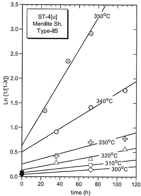
Fig. 7. Plot of first-order rate function versus time at designated temperatures for sample ST-4[u] (Type-IIS kerogen).
